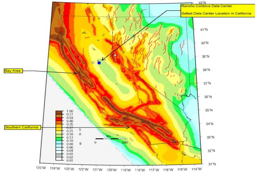
Figure 40. Map of 1-hertz spectral acceleration (SA) for 2-percent probability of exceedance in 50 years in California in standard gravity (g). Red lines are fault sources used in the model.
